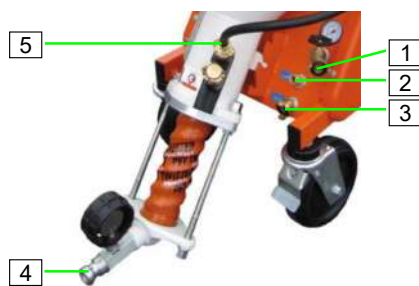
Abb. 18: Anschlüsse
